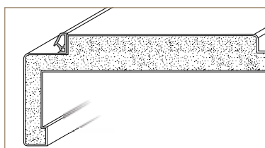
SMS CLOSED FRAME WITH ROUNDED CASE PROFILES AND ROUNDED PANEL LINING
